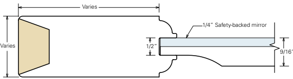
Sample cross section (one-sided mirror door)
